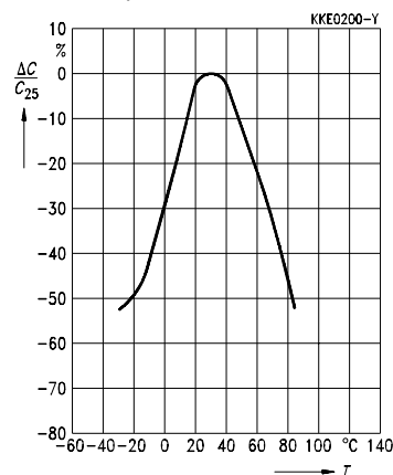
Typical characteristics of Z5U-MLCC 2) Capacitance change \Delta C/C_{25} versus temperature T
